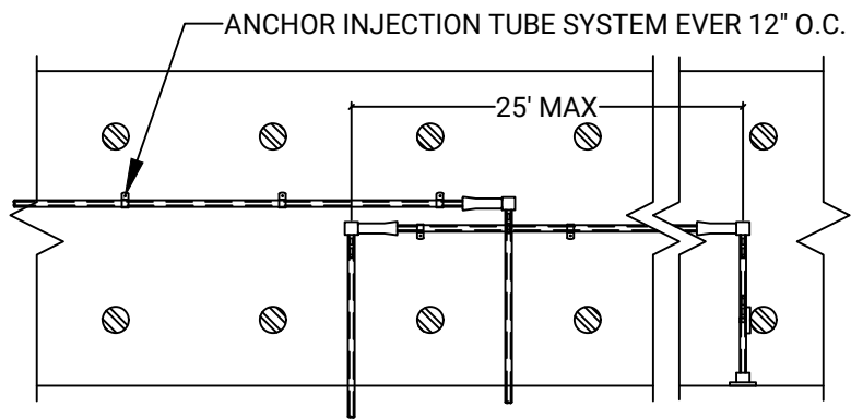
1 AERIEL VIEW OF CONCRETE STRUCTURE N.T.S.
